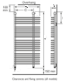
Dimensions and fixing centres (all models)
